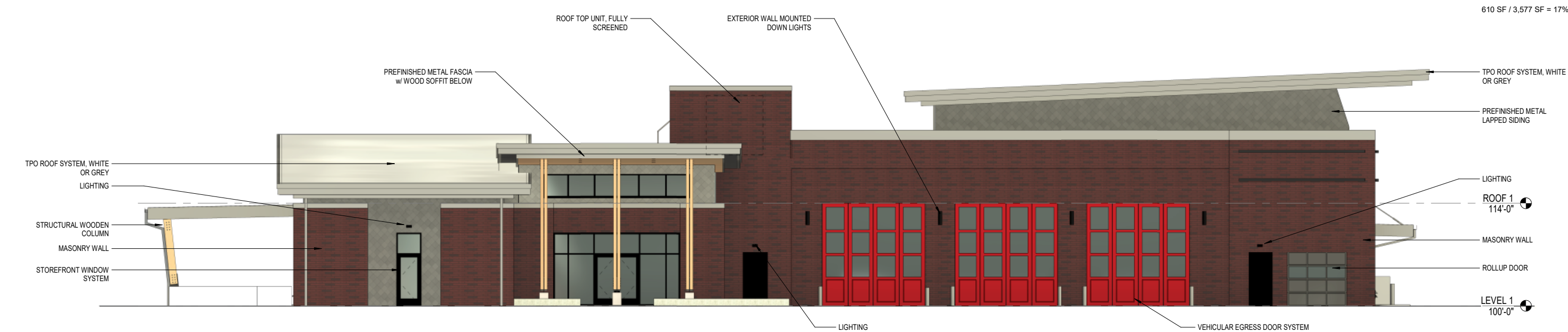
1 SOUTH ELEVATION 1/8" = 1'-0"
