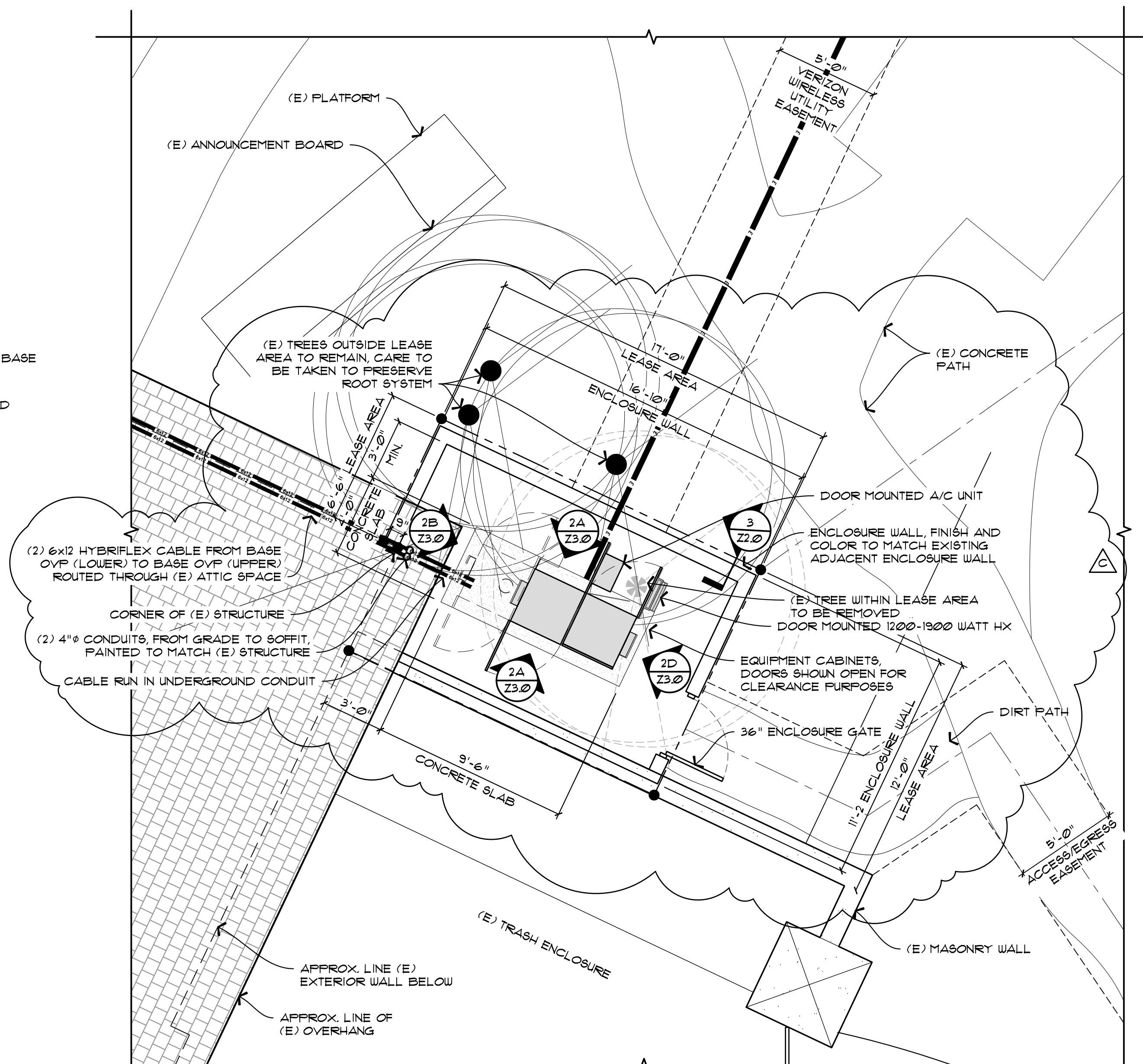
ENLARGED EQUIPMENT CABINET PLAN SCALE: 1/4" = 1'-0" RE: 1/21 TRUE NORTH 0' 1' 2' 4' 8'
