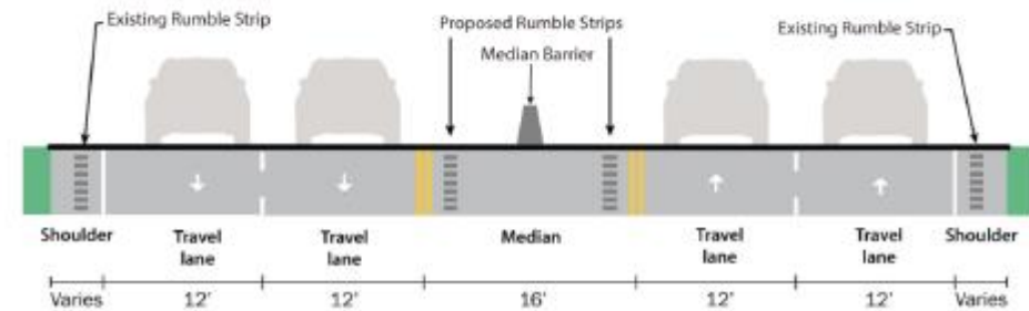
Figure X. US 287 Proposed Median Barrier Cross Section
