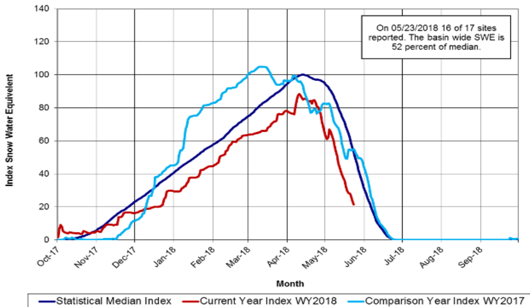
Upper Colorado River Headwater Basin Snotel Tracking Aggregate of 17 Snotel Sites in the Upper Colorado Headwater Basin
